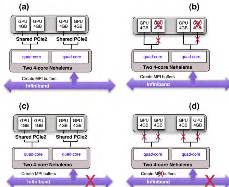
Fig. 10. Description of the four types of tests performed on the cluster of 48 Tesla S1070 depicted in Fig. 9.
