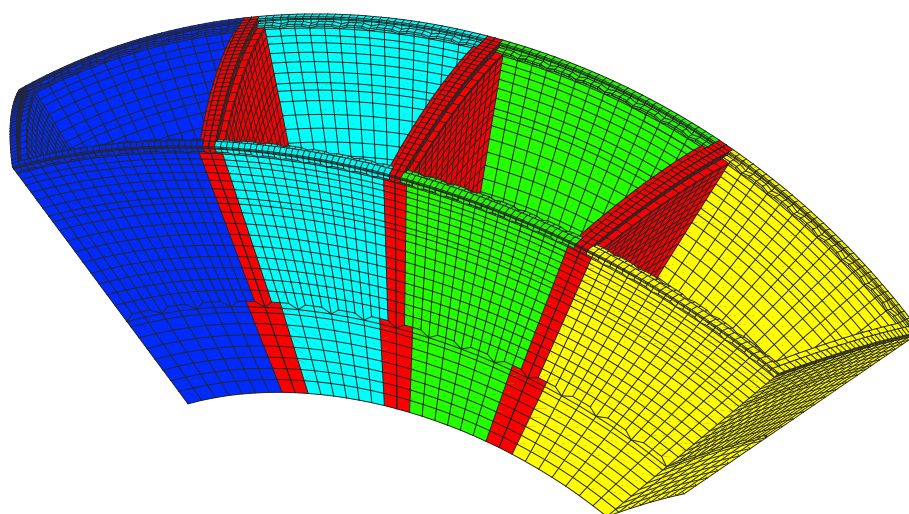
Fig. 3. Outer (red) and inner (other colors) elements for part of the mesh of Fig. 1. Elements in red have at least one point in common with an element from another slice and must therefore be computed first, before initiating the non-blocking MPI communications. The picture also shows that the mesh is unstructured because we purposely increase the size of the elements with depth based on a ‘mesh doubling brick’. This is done because seismic velocities and therefore seismic wavelengths increase with depth in the Earth. Therefore, larger elements are sufficient to sample them; they lead to a reduction in the computational cost. Here for clarity only the cut planes that define the mesh slices have been drawn; but in reality the mesh is filled (see Fig. 1, left, and Fig. 6). (For interpretation of the references to colour in this figure legend, the reader is referred to the web version of this article.)
