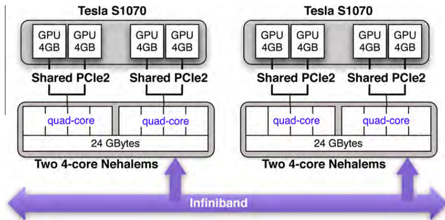
Fig. 9. Description of the cluster of 48 Tesla S1070 used in this study. Each Tesla S1070 has four GT200 GPUs and two PCI Express-2 buses (i.e., two GPUs share a PCI Express-2 bus). The GT200 cards have 4 GB of memory, and the memory bandwidth is 102 GB/s with a memory bus width of 512 bit. The Teslas are connected to BULL Novascale R422 E1 nodes with two quad-core Intel Xeon X5570 Nehalem processors operating at 2.93 GHz. Each node has 24 GB of RAM. The network is a non-blocking, symmetric, full duplex Voltaire InfiniBand double data rate (DDR) organized as a fat tree.
