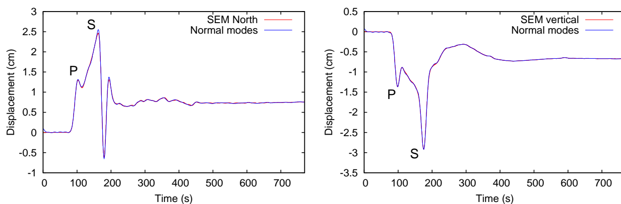
Fig. 8. Numerical time variation of the components of the displacement vector at station 'ST04' of the 'BANJO' seismic recording array in Bolivia during the magnitude 8.2 earthquake of June 9, 1994. The earthquake occurred at a depth of 647 km. Left: North–South component, Right: vertical component. The red line shows the spectral-element CUDA + MPI solution and the blue line shows the independent quasi-analytical reference solution obtained based on normal-mode summation. The agreement is excellent, which further validates our CUDA + MPI implementation. The pressure (P) and shear (S) waves are accurately computed and the large 6.6 mm and 7.3 mm static offsets observed on the vertical and North–South components, respectively, are correctly reproduced. Note that the quasi-analytical reference solution obtained by normal-mode summation contains a small amount of non-causal numerical noise (see e.g. the small oscillations right after t = 0 on the North component, while the first wave arrives around 100 s). Therefore, the small discrepancies are probably due to the reference solution.
