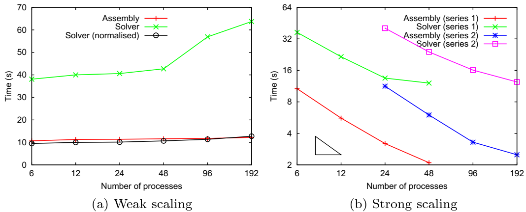
Fig. 1. Weak and strong scaling of FEAST on the Tibidabo ARM cluster, showing absolute time in seconds. A horizontal line corresponds to perfect weak scaling. Normalised timings are obtained by dividing the measured time by the number of solver iterations. Strong scaling is depicted as a log-log plot of absolute time, so that a line with slope -1 , as shown by the small black triangle, corresponds to perfect strong scaling.
