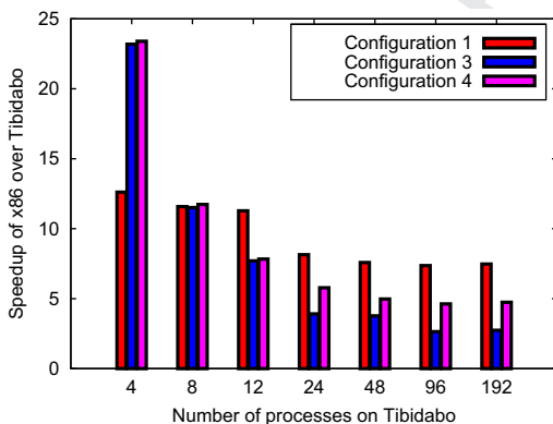
(a) Speedup LiDong over Tibidabo (time per time step)
