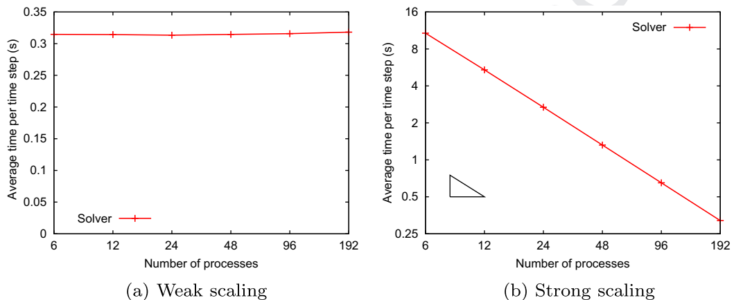
Fig. 2. Weak and strong scaling of HONEI_LBM on the Tibidabo ARM cluster, showing average time per time step in seconds. A horizontal line corresponds to perfect weak scaling. Strong scaling is depicted as a log-log plot of average time per time step, so that a line with slope -1 , as shown by the small black triangle, corresponds to perfect strong scaling.
