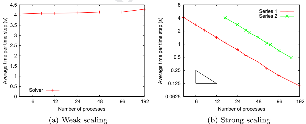
Fig. 3. Weak and strong scaling of SPECFEM3D_GLOBE on the Tibidabo ARM cluster, showing average time per time step in seconds. A horizontal line corresponds to perfect weak scaling. Strong scaling is depicted as a log-log plot of average time per time step, so that a line with slope -1 , as shown by the small black triangle, corresponds to perfect strong scaling.
